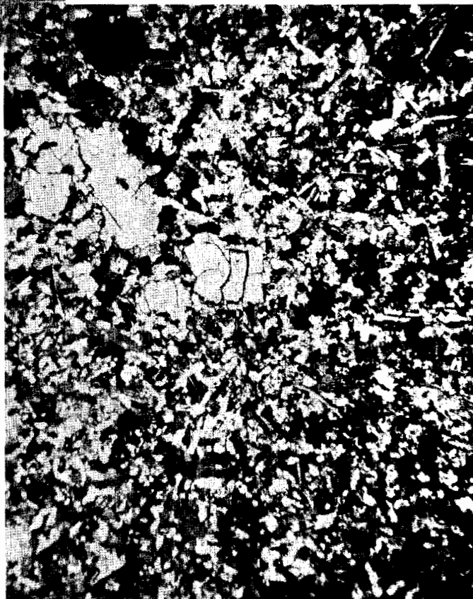
Figure 2. Photomicrograph of 15548,4. Width about 3 mm. a) transmitted light; b) crossed polarizers.
