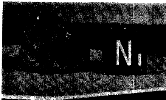
Figure 1. Pre-chip view of 15666. S-71-49757
