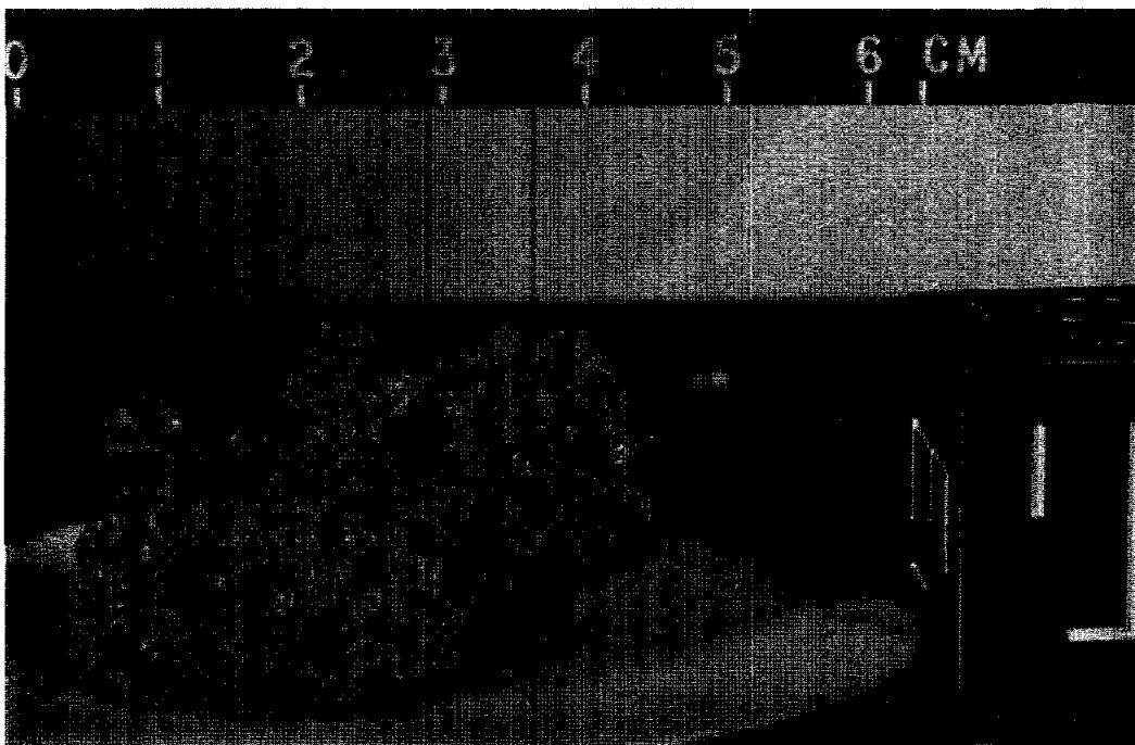
Figure 1. Macroscopic, pre-split view of 15630. S-71-49269
