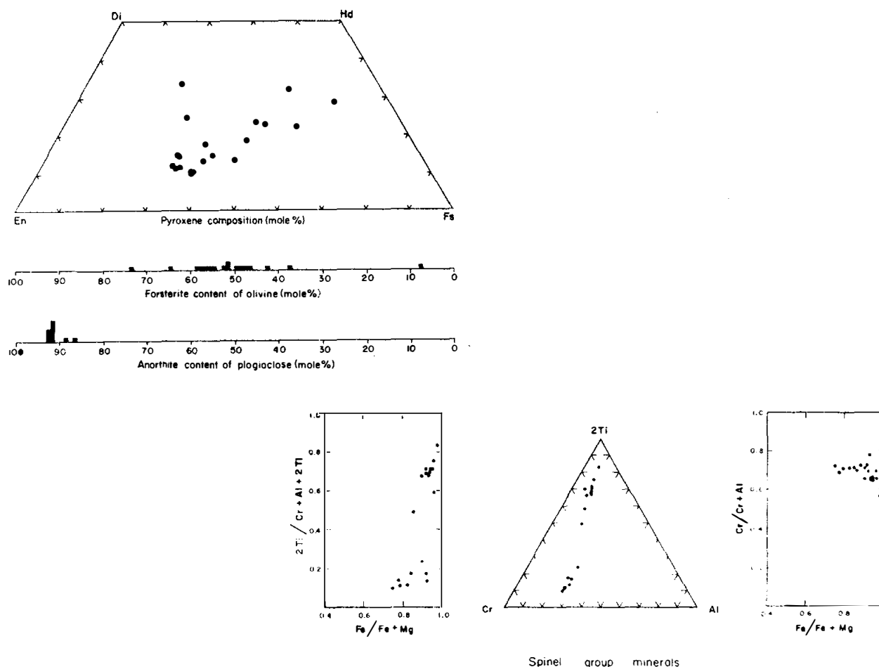
Figure 3. Chemistry of minerals in 15633 (Dowty et al. , 1973b).
