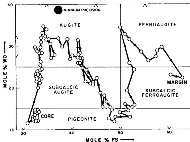
Figure 6. Pyroxene zoning profile (Mason, 1972).
