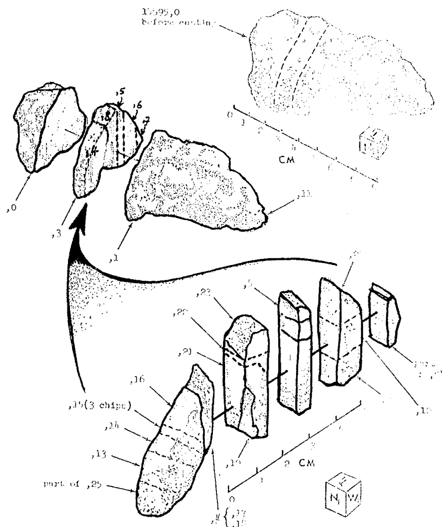
Figure 8. Cutting of 15595.
