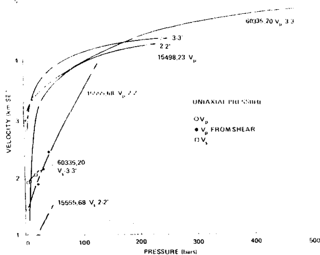
Figure 20. Seismic velocity as a function of pressure (Warren et al., 1973).
