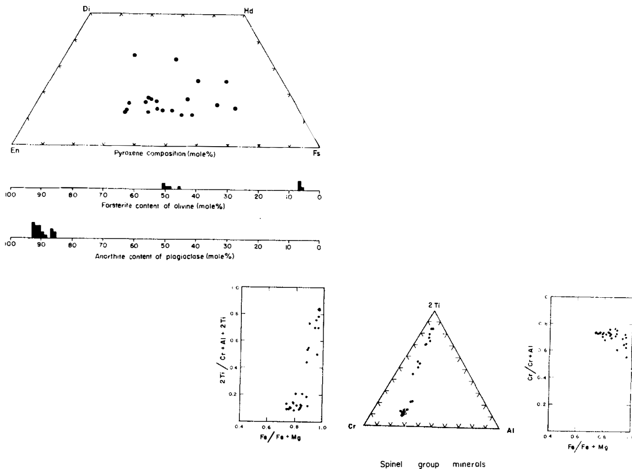
Figure 3. Chemistry of minerals in 15641 (Dowty et al., 1973b).
