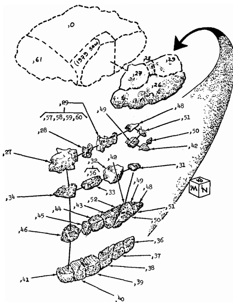
Figure 4. Dissection of 15495.
