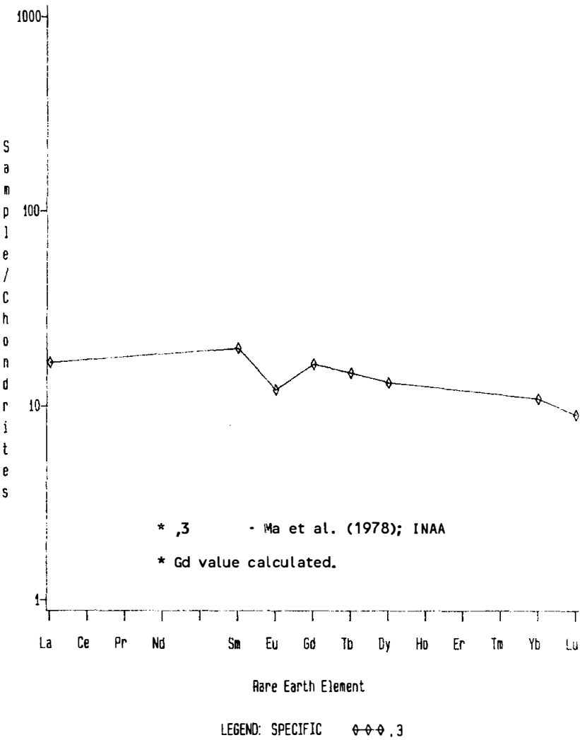
Figure 3. Rare earths in 15612.
