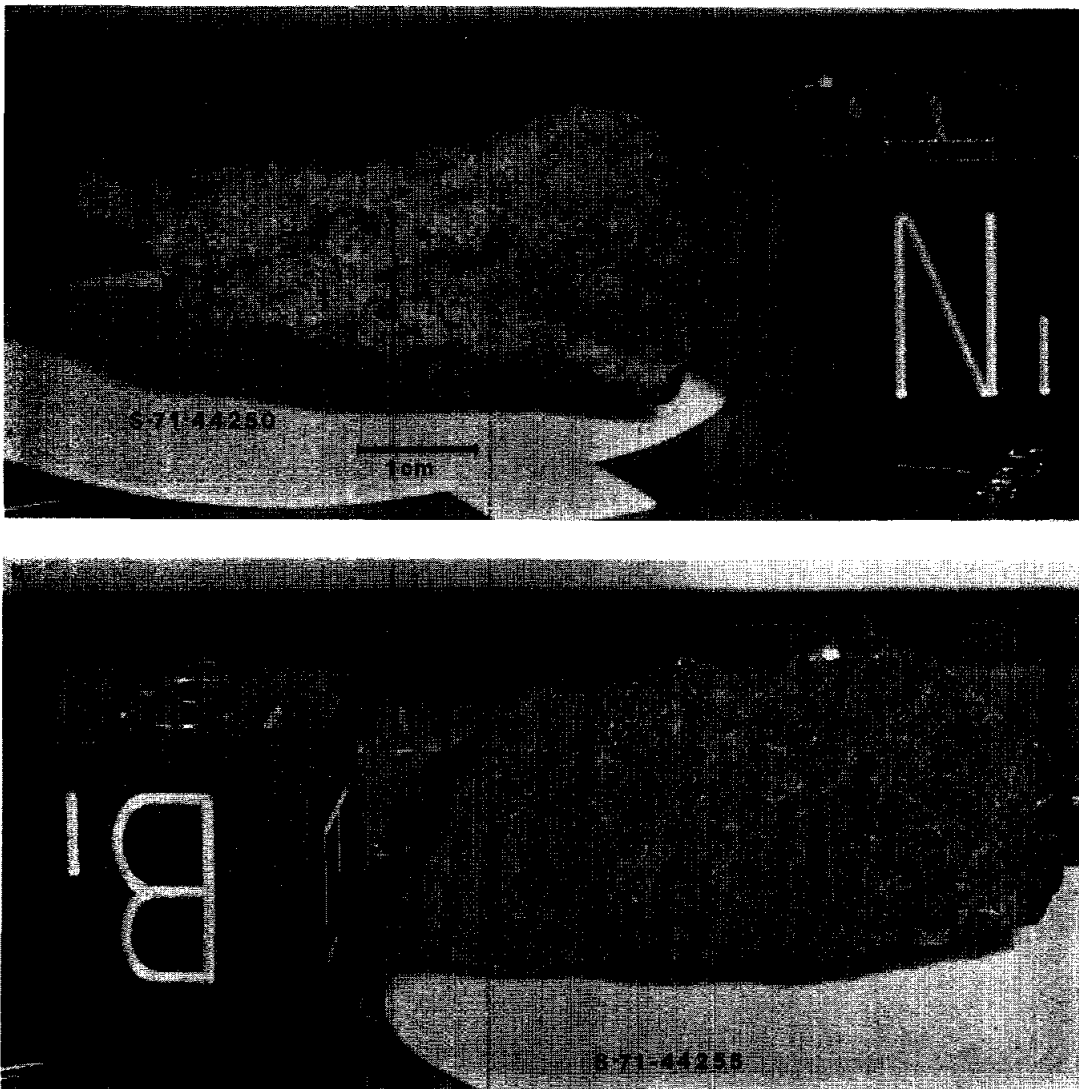
Figure 1. Macroscopic views of original sample, showing the pale-colored coat on "N" side.
