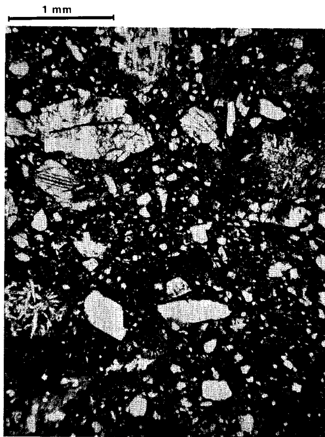
Figure 2. Photomicrograph of breccia matrix of 15558,9, transmitted light.
