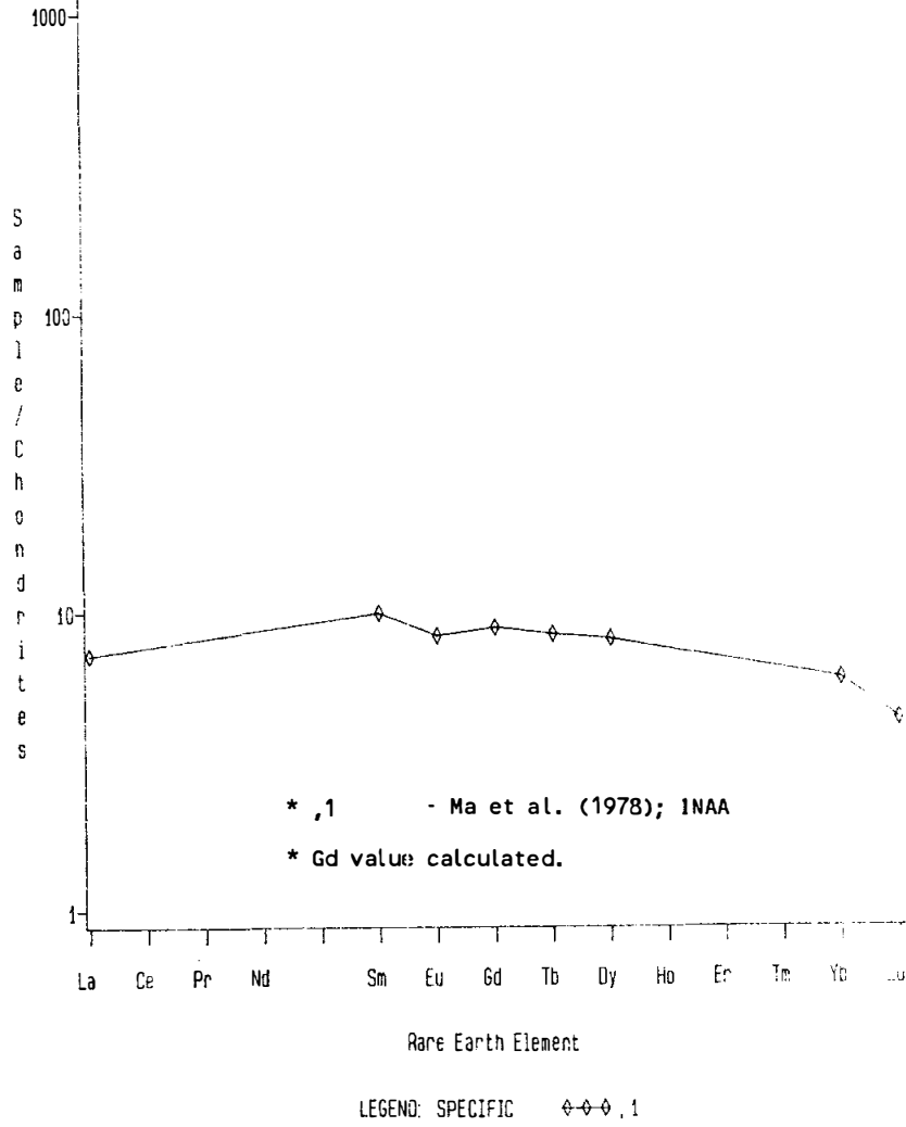
Figure 3. Rare earths in 15634.
