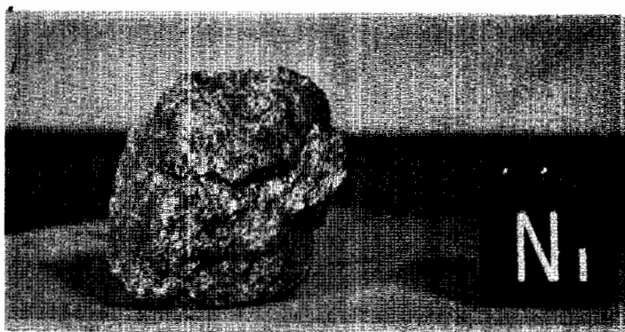
Figure 1. Pre-chip view of 15648. S-71-49773
