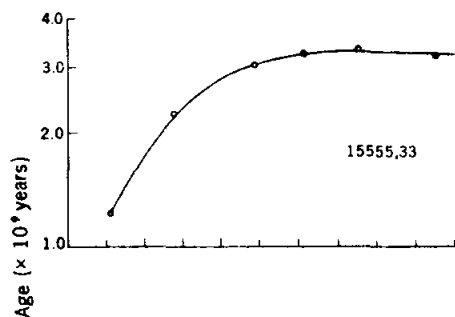
Figure 12. Ar release diagrams. (a) Alexander et al. (1972); (b) Podosek et al. (1972); (c) Husain et al. (1972a).
