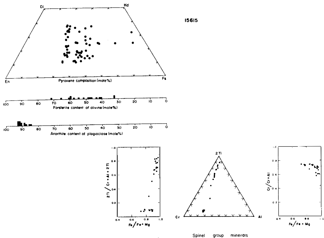
Figure 3. Chemistry of minerals in 15615 (Dowty et al. , 1973b).
