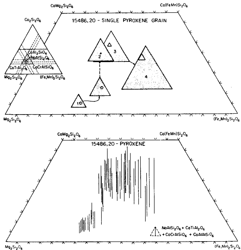
Figure 3. Compositions of pyroxenes in 15486,20 (Albee et al. 1972).
