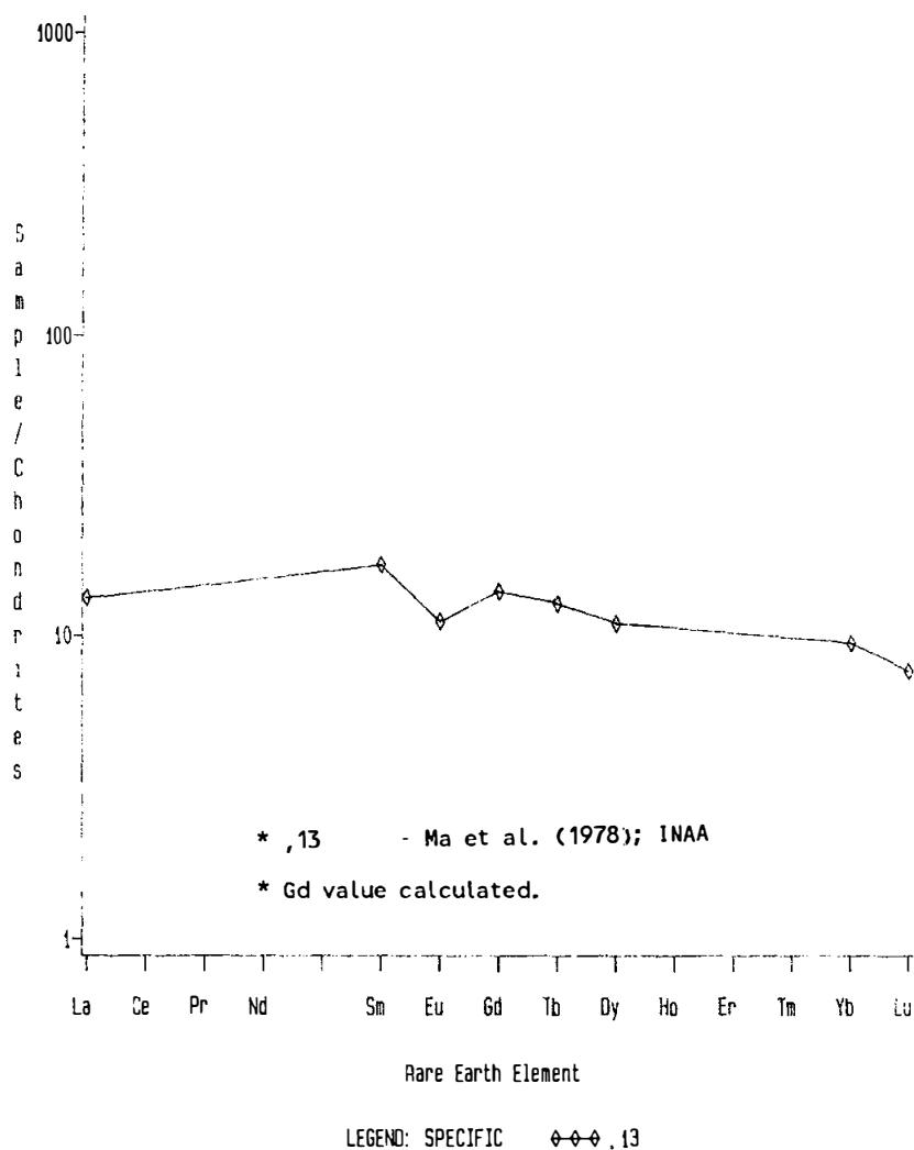
Figure 4. Rare earths in 15641.
