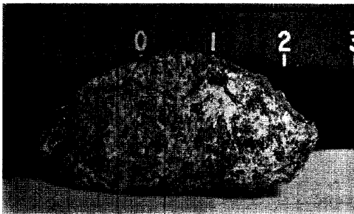
Figure 1. Pre-chip, macroscopic view of 15547. S-71-44969
