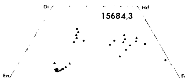
Figure 5. Compositions of pyroxenes in 15684 pyroxene-phyric basalt clast (Schaal and Horz, 1977).
