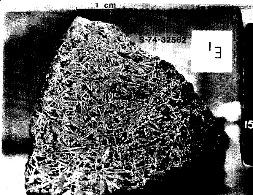
Figure 1. Sawn face of W end piece ,21, showing pigeonite phenocrysts.
