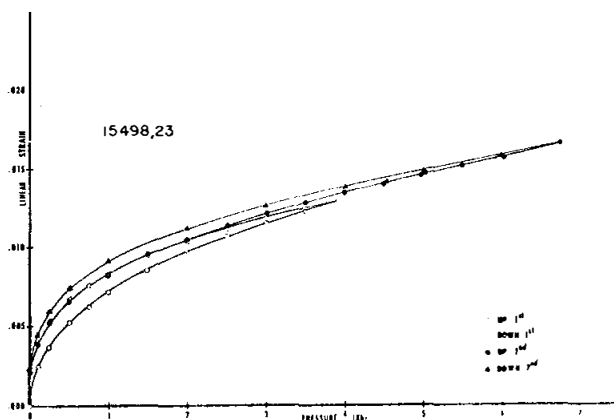
Figure 9. Linear strain vs. pressure for 15498,23 (Trice et al. , 1974).
