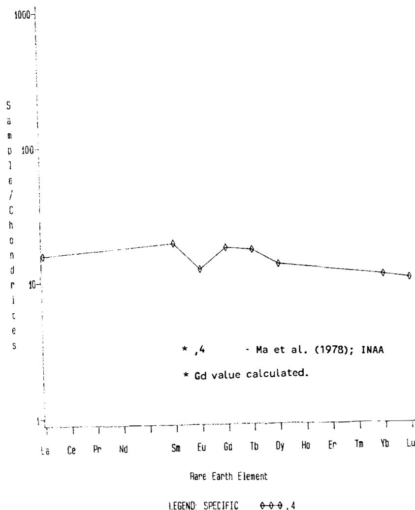
Figure 4. Rare earths in 15623.
