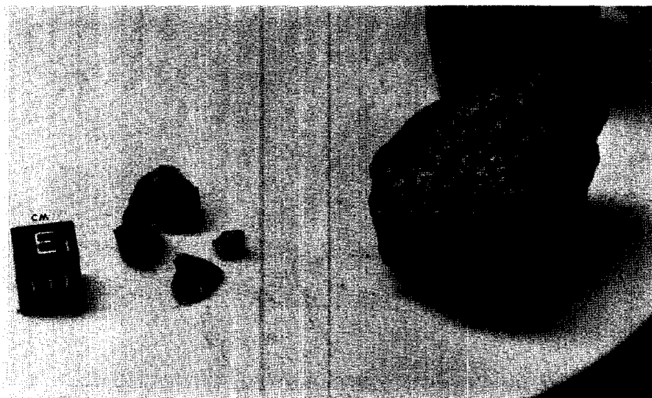
Figure 1. Post chip view of 15647. S-71-56353
