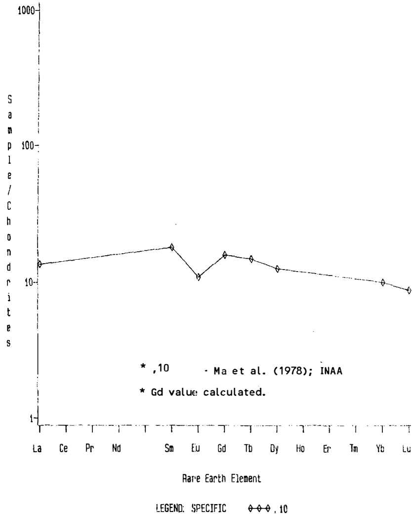
Figure 3. Rare earths in 15664.
