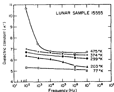
Dielectric constant of sample 15555,88 as a function of frequency and temperature.
