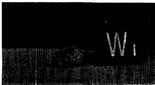
Figure 1. Sample 15681. S-71-49870
