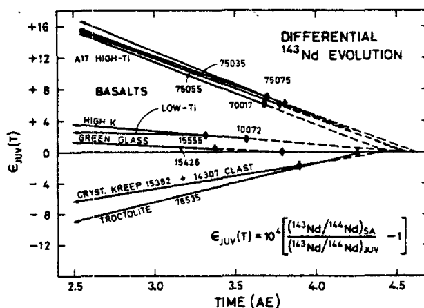
The differential ^{143}\text{Nd} evolution \epsilon_{\text{JUV}}(T) relative to Juvinas is shown for four Apollo 17 basalts, one each Apollo 11 and 15 basalt, green glass 15426, one each KREEP basalt and clast and troctolite 76535.
