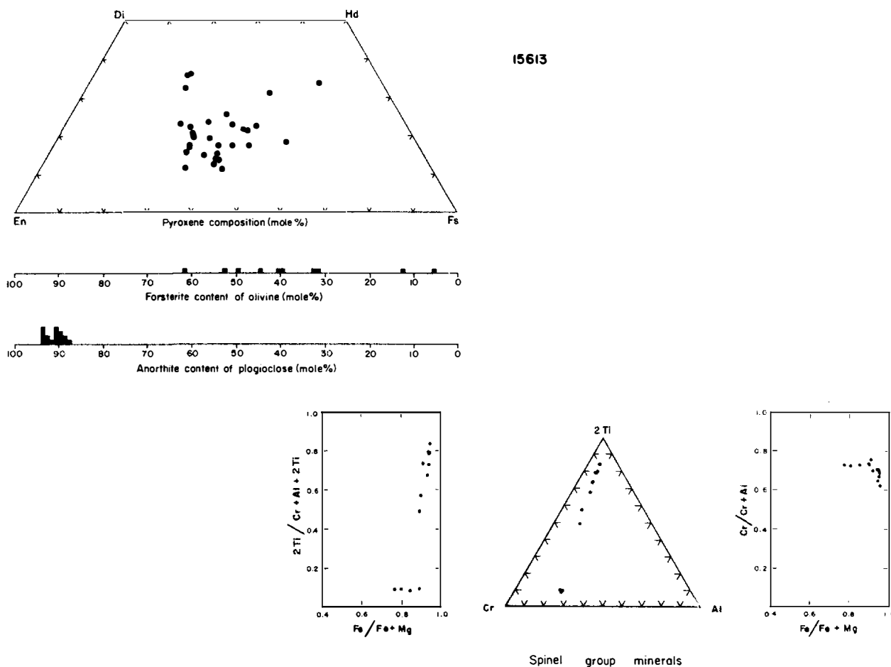
Figure 3. Chemistry of minerals in 15613 (Dowty et al. , 1973b).
