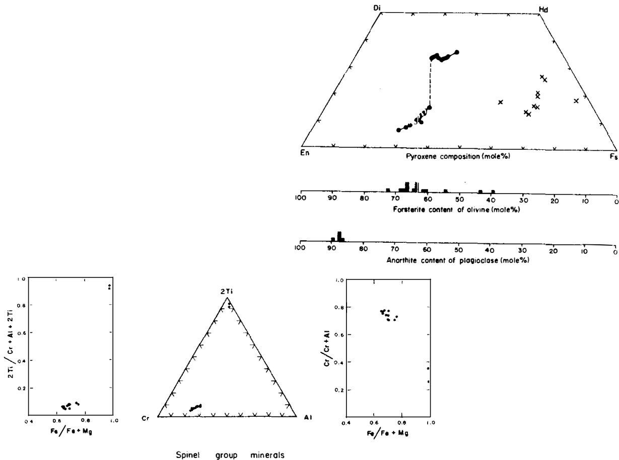
Figure 3. Compositions of minerals in 15666. On pyroxene plot, dots are for a phenocryst, x's are groundmass (Dowty et al., 1973b).
