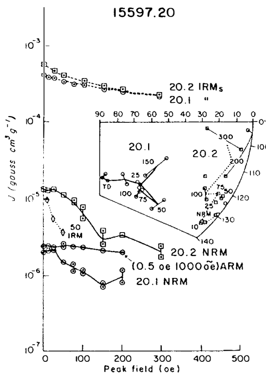
Figure 9. AF demagnetization of 15597,20. Inset is directional changes. (Fuller et al., 1979).
