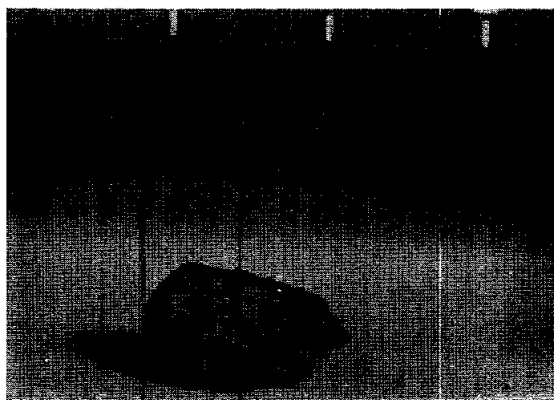
Figure 1. Pre-split view of 15608. S-71-44966
