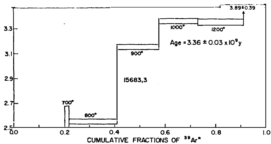
Figure 4. ^{40}\text{Ar} - ^{39}\text{Ar} plateau age for 15683 (Husain, 1974).
