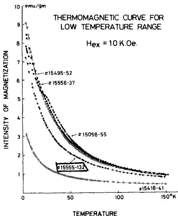
Figure 17. Thermomagnetic curve (Nagata et al. , 1973).
