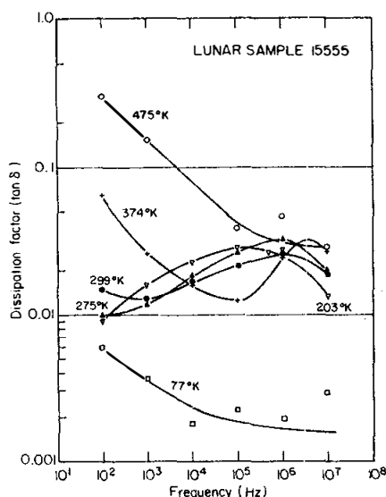
Dielectric losses in sample 15555,88 as a function of frequency and temperature.
