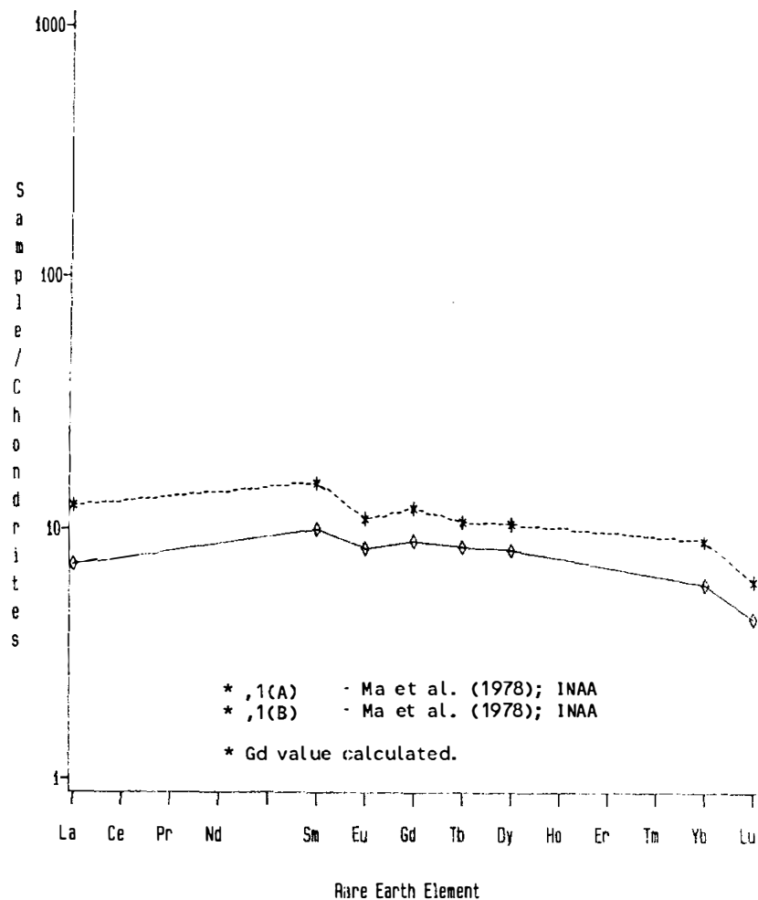
Figure 3. Rare earths in 15639.
