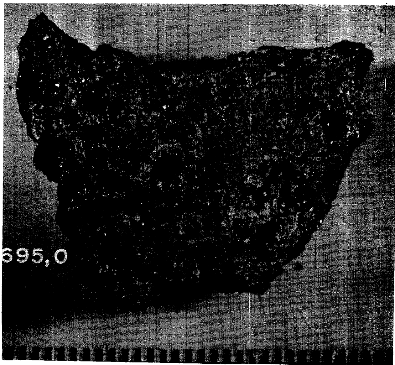
Figure 1. Sample 15695. S-75-33962
