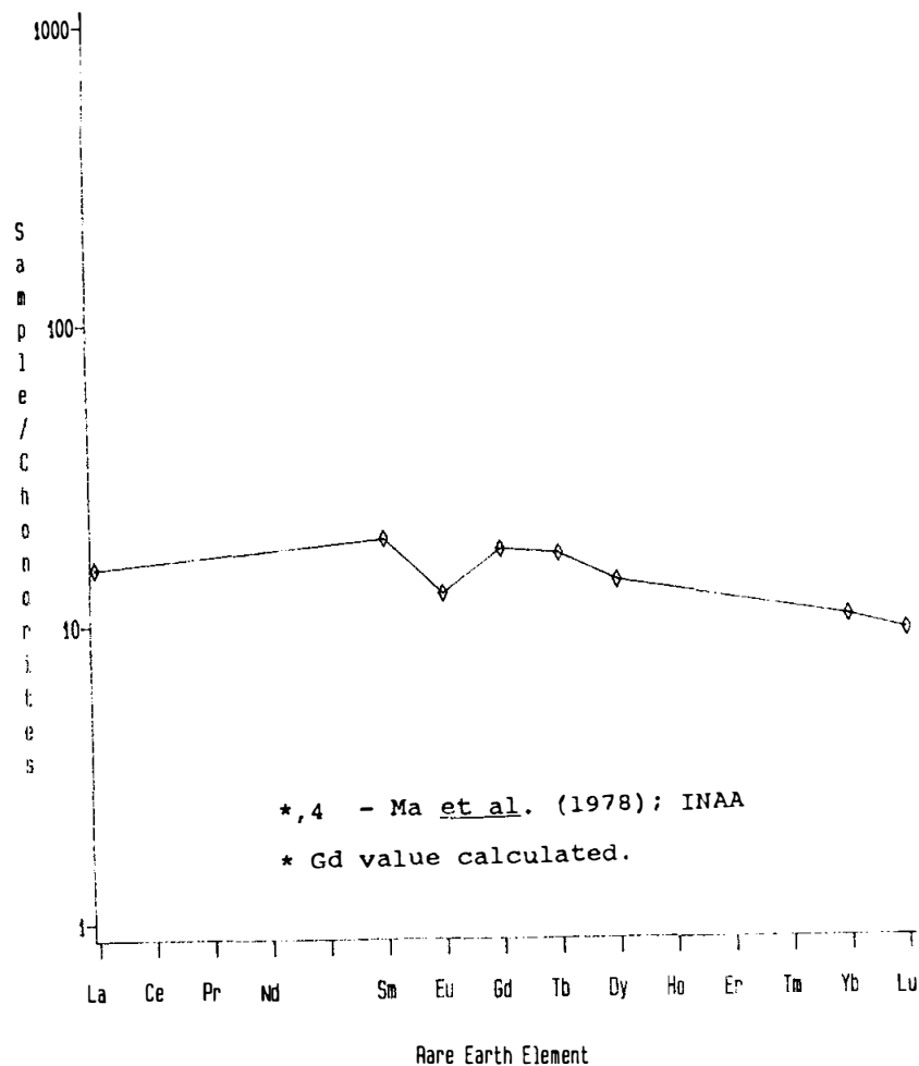
Figure 4. Rare earths in 15669.
