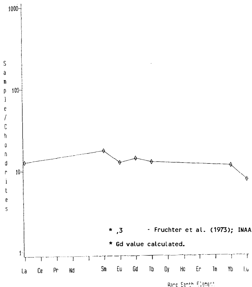
Figure 3. Rare earths in 15674.
