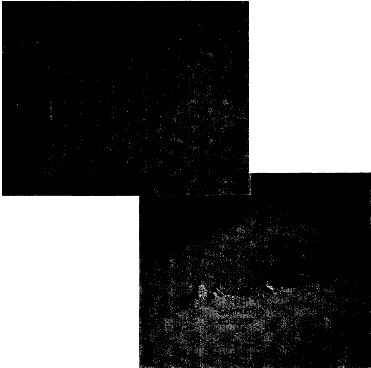
Figure 1. Sampling locations for 15485, 15486, and 15499 from a boulder on the south rim of Dune Crater.
