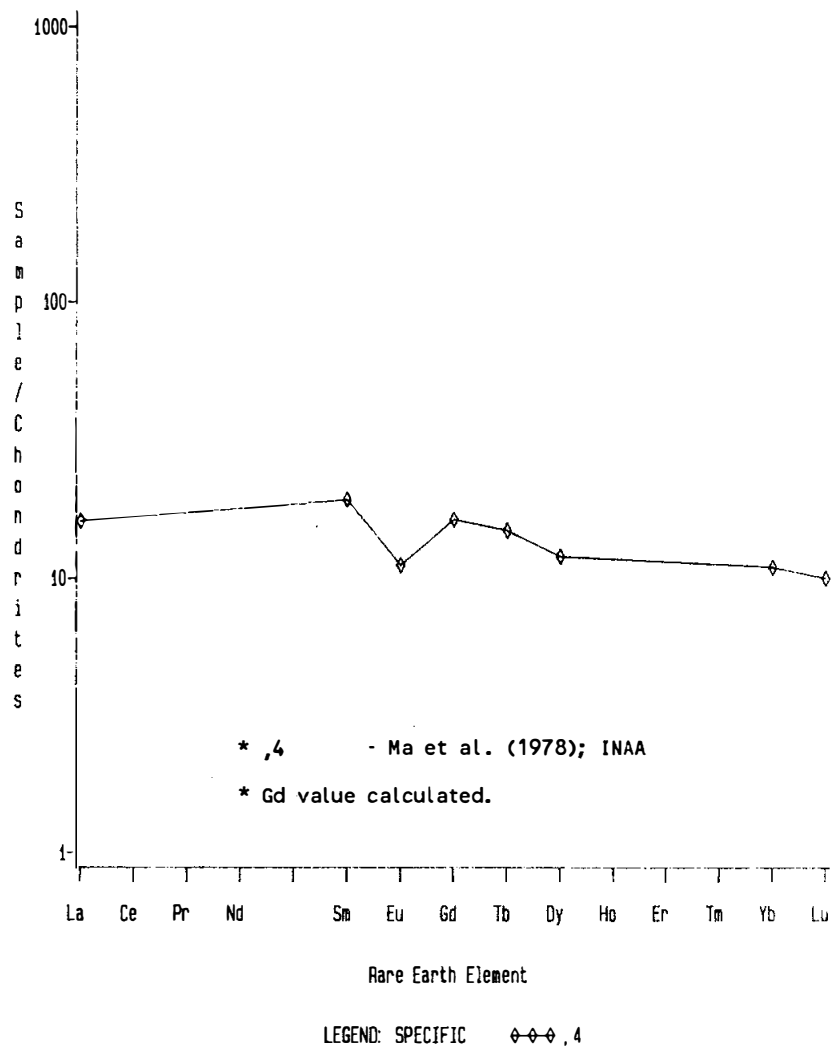
Figure 3. Rare earths in 15616.
