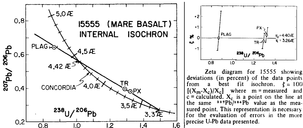
U-Pb internal isochron for 15555. If, on the basis of Rb-Sr data a lower intersection at 3.3 AE is chosen then the isochron (passing through the center of total rock point) yields an upper intersection at the magic point 4.42 AE. A best fit line yields 3.26 AE and 4.40 AE respectively for lower and upper intersections.
