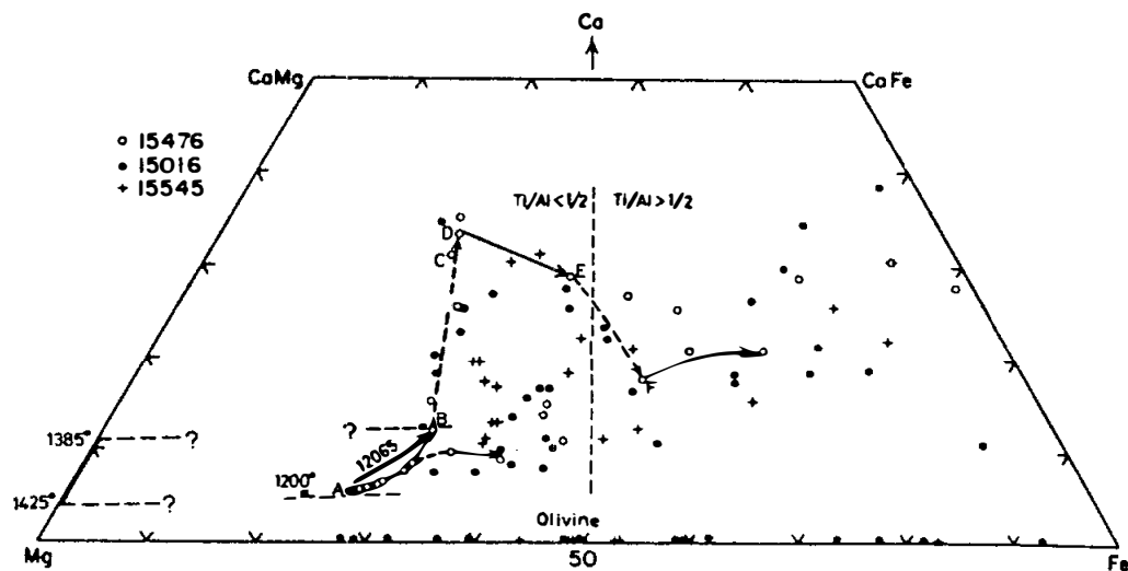
Figure 3. Compositions of pyroxenes in 15476 (open circles) and two other Apollo 15 mare basalts. Solid lines show continuous, dashed lines show discontinuous, zoning in a single crystal (Kushiro, 1973).
