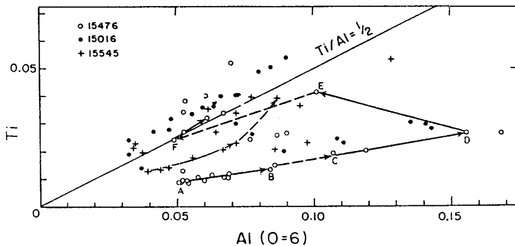
Figure 4. Ti-Al variations in pyroxenes in 15476 (open circles) and two other Apollo 15 mare basalts (Kushiro, 1973).
