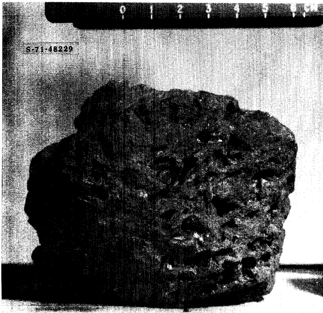
Figure 1. Macroscopic view of "N" face of 15495.
