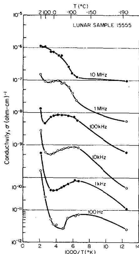
Electrical conductivity of sample 15555,88 as a function of frequency and temperature.
