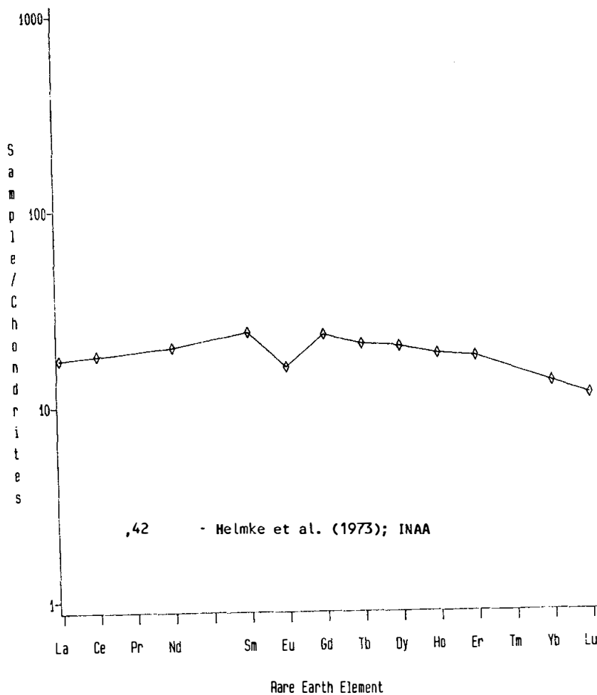
Figure 4. Rare earths in 15557.
