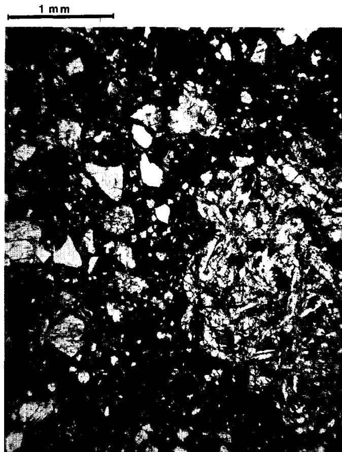
Figure 2. Photomicrograph of matrix of 15505,48, transmitted light.
