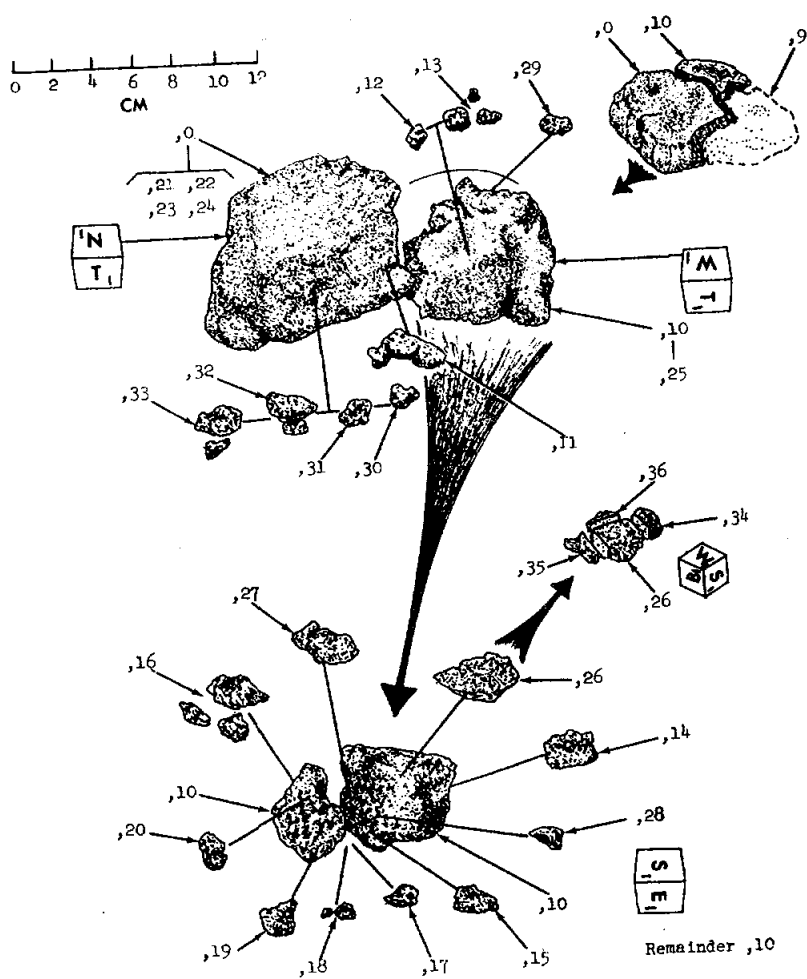
Figure 11. Dissection of 15499.
