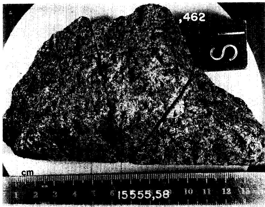
Figure 3. Close-up showing vuggy nature.
