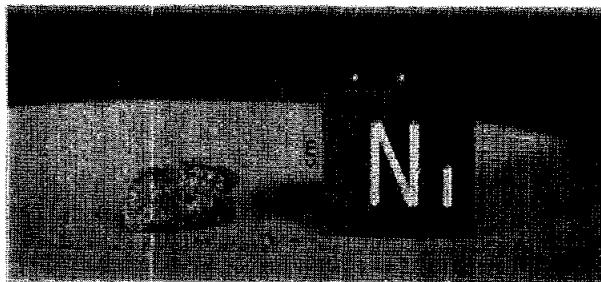
Figure 1. Sample 15654. S-71-49765
