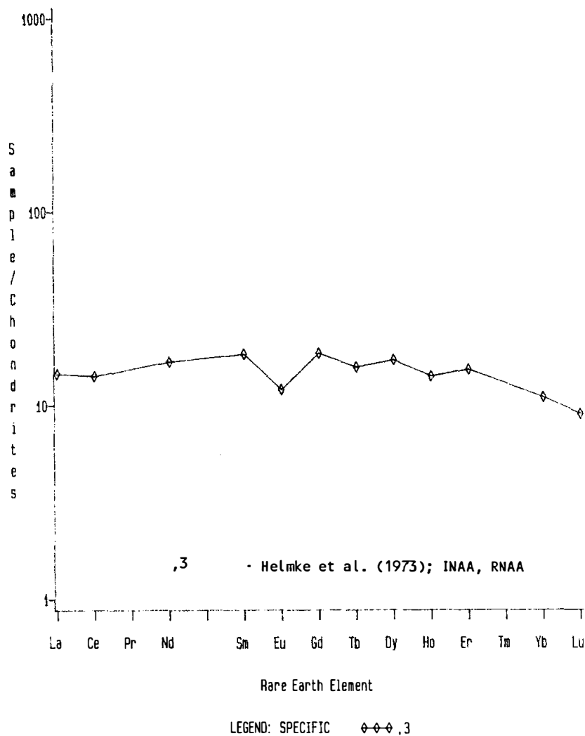
Figure 4. Rare earths in 15665.
