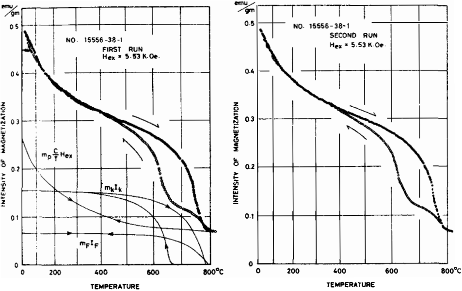
Thermomagnetic curve of Apollo 15 basalt No. 15556-38 in temperature range from 20 to 820 °C.
