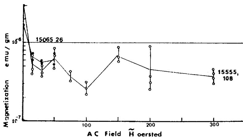
Figure 16. AF demagnetization. (a) Collinson et al. (1973); (b) Dunn and Fuller (1972); (c) Hargraves and Dorety (1972).
