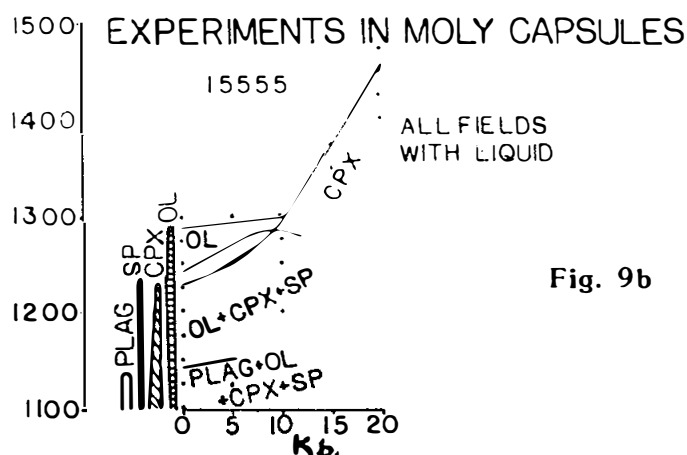
Figure 9. Experimental phase petrology. (a) and (b) Longhi et al. (1972); (c) Humphries et al. (1972).
