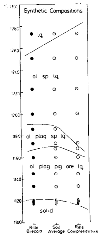
Figure 3. Experimental results of crystallization of a synthetic 15558 composition (black dots) and basalt and soil samples for comparison (Humphries et al. , 1972).
