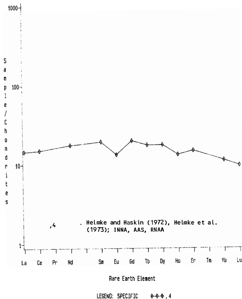
Figure 4. Rare earths in 15647,4.
