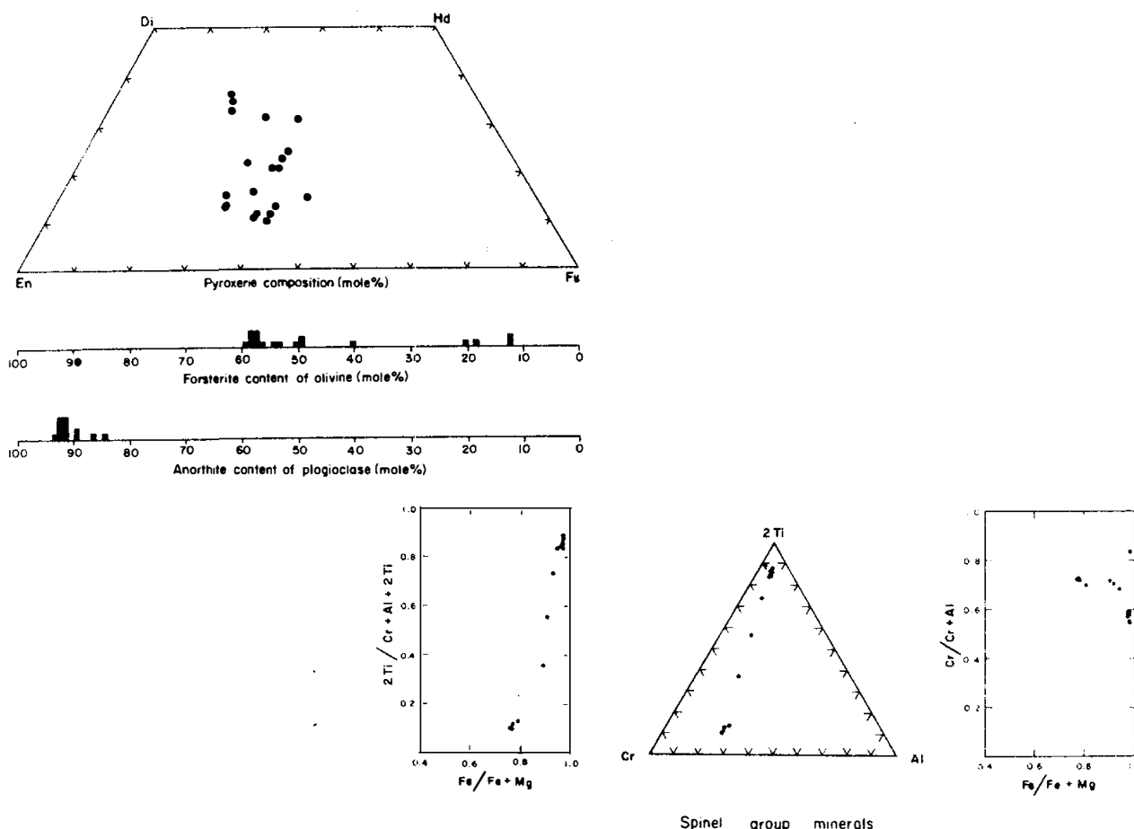
Figure 3. Chemistry of minerals in 15643 (Dowty et al. , 1973b).
