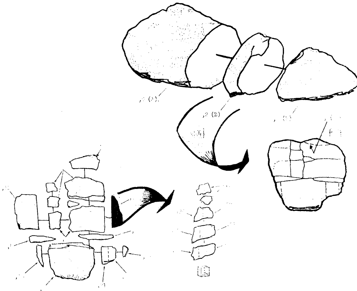
Figure 5. Subdivisions of 15557.
