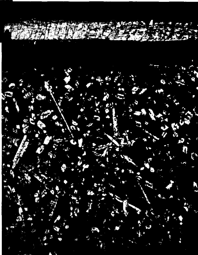
Figure 2. Photomicrographs of 15597,12, showing small acicular phenocrysts, opaque glassy groundmass, small vesicles, and part of a twinned megacryst. a) transmitted light; b) crossed polarizers.
