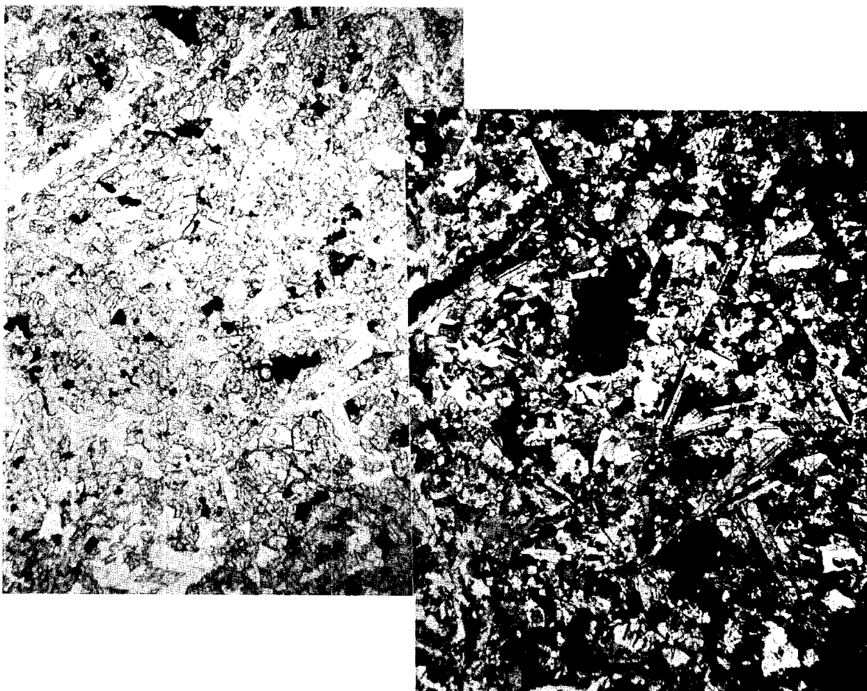
Figure 2. Photomicrographs of 15598, 10. Widths about 3 mm. a) transmitted light; b) crossed polarizers.
