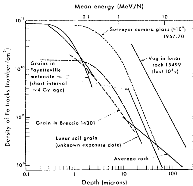
Figure 8. Track density profile of Hutcheon et al. (1972) (from Price et al. , 1973).
