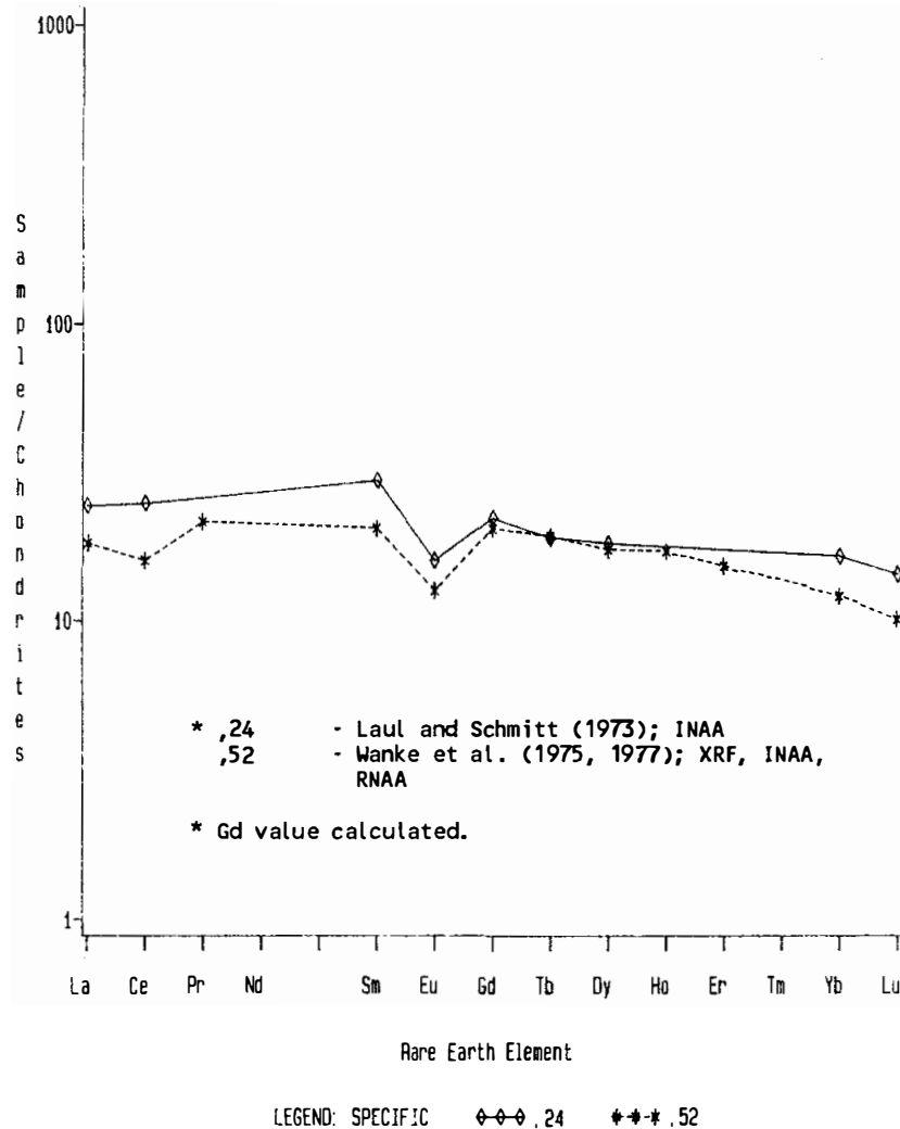
Figure 3. Rare earth abundances for 15495.
