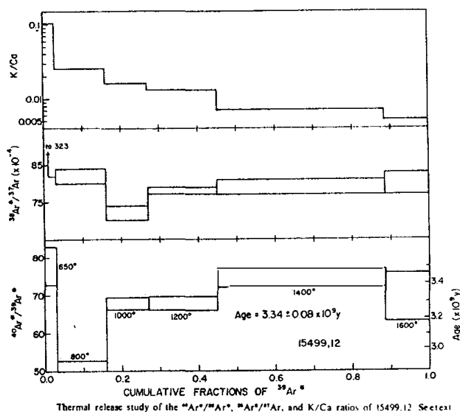
Figure 7. Ar release diagram (Husain, 1974).
