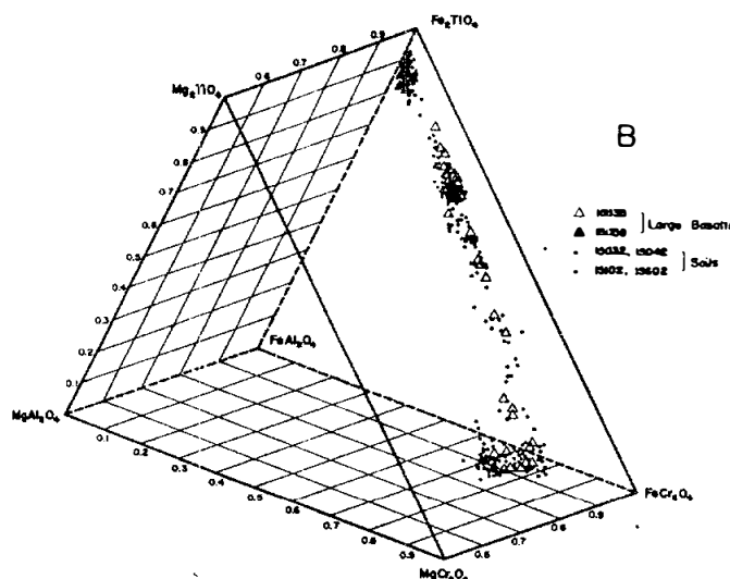
Figure 3. Compositions of spinel group minerals in 15535 (open triangles) and other Apollo 15 samples (Haggerty, 1972c).
