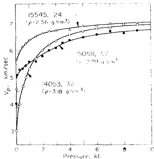
Figure 6. Elastic wave velocities in 15545 and other basalt samples (Mizutani and Newbigging, 1973).
