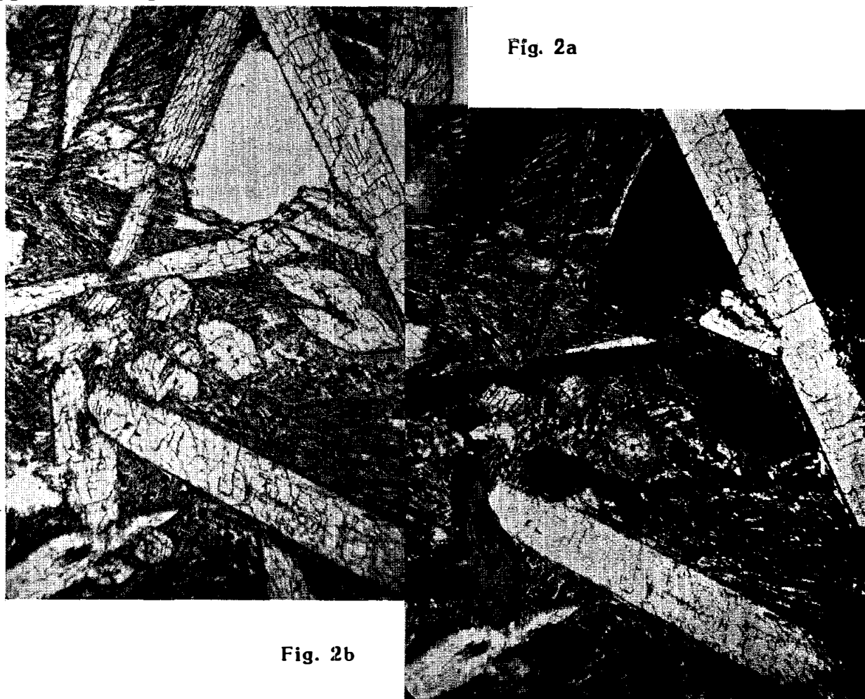
Figure 2. Photomicrographs of 15596,12, showing pigeonite phenocrysts with their augite rims, hollow cross-sections, vug, and spherulitic groundmass containing opaques. Widths about 3 mm. a) transmitted light; b) crossed polarizers.
