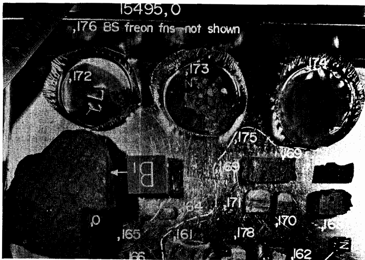
Figure 5. Subsplits of 1979 saw cut and remainder of ,0.
