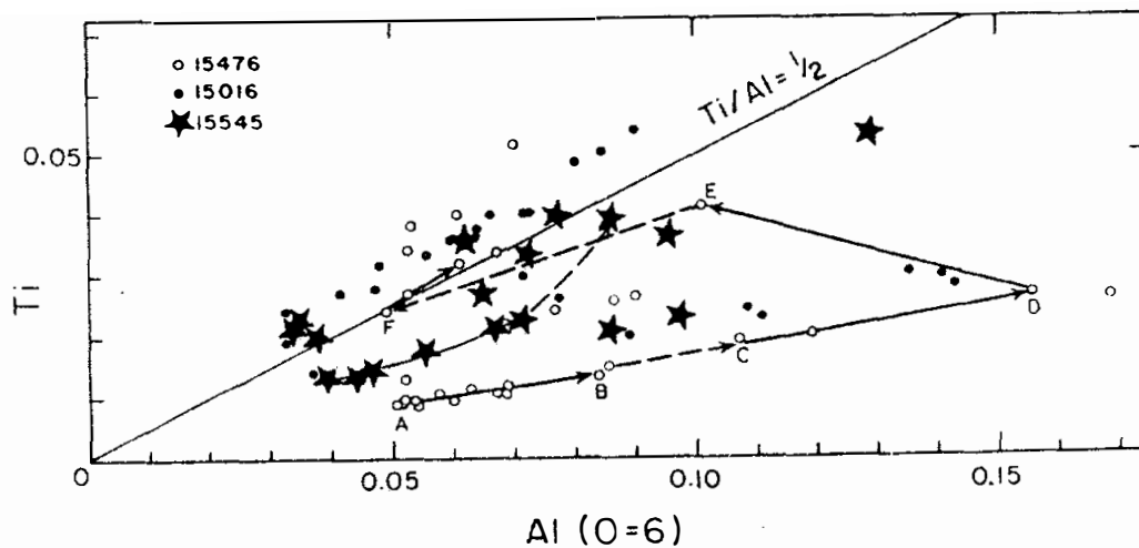
Figure 4. Ti vs. Al for pyroxenes in 15545 and other samples (Kushiro, 1973).
