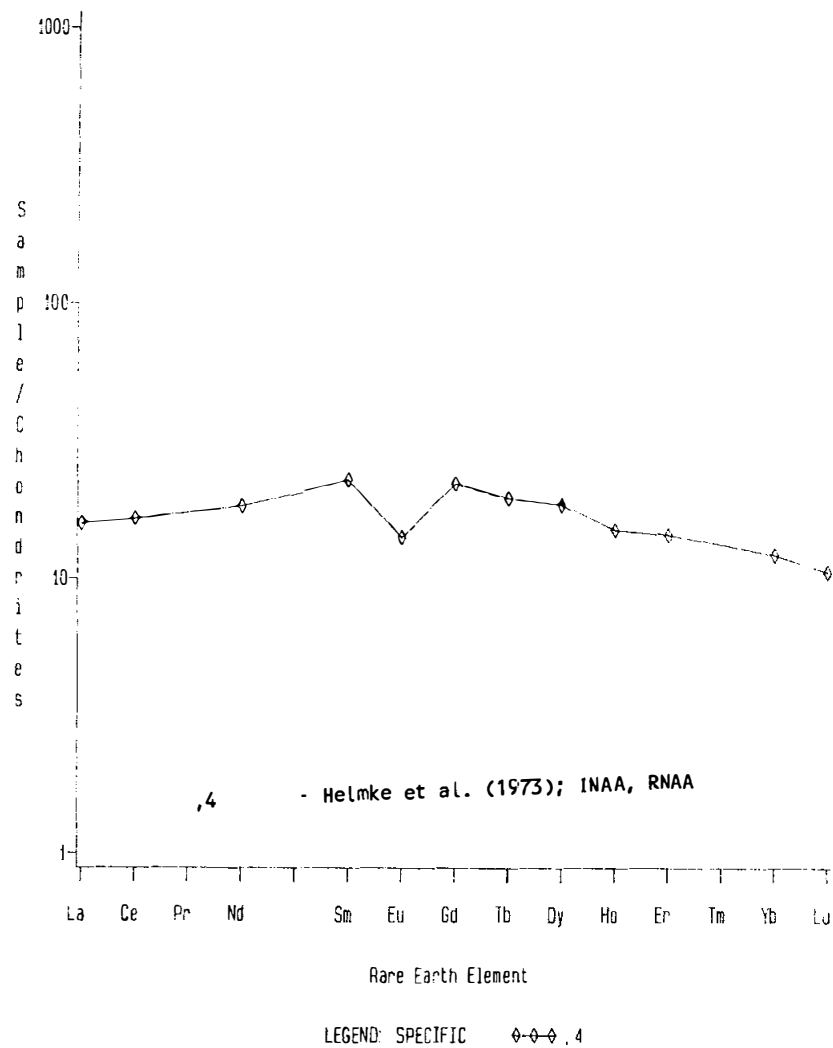
Figure 3. Rare earths in 15683.
