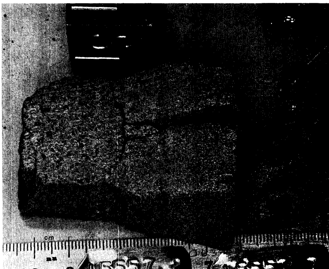
Figure 2. Part of sawn slab.
