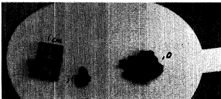
Figure 1. Post-chip view of 15615. S-71-56171
