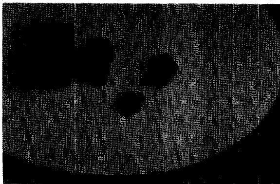
Figure 1. Post-chip view of 15613. Medium-sized chip is ,1.
