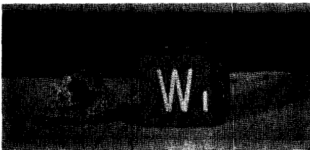
Figure 1. Sample 15655. S-71-49746
