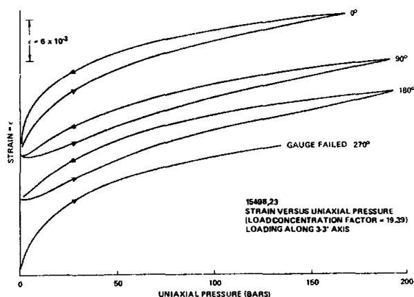
Figure 8. Strain results under axial loading for 15498,23 (Warren et al. , 1973).
