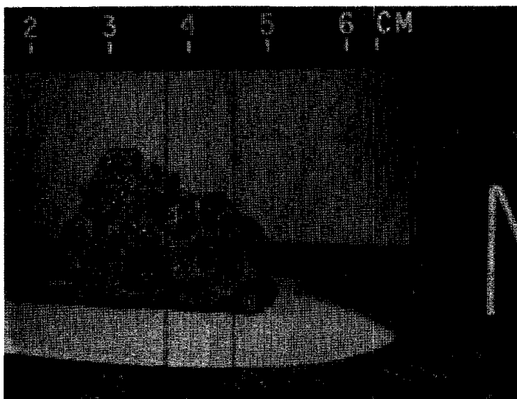
Figure 1. Pre-chip view of 15616. S-71-49120
