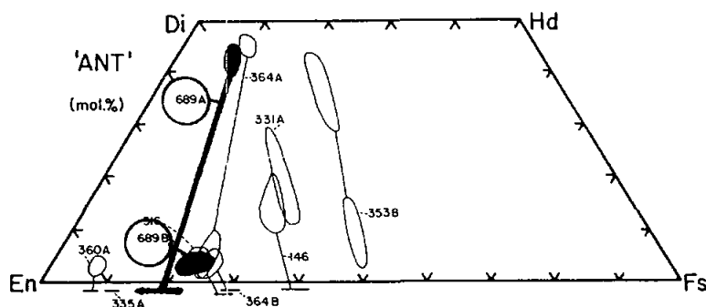
Figure 3. Pyroxene and olivine compositions in two clasts for 15689. "A" is the pristine norite. "B" is subophitic (Steele et al., 1977).
