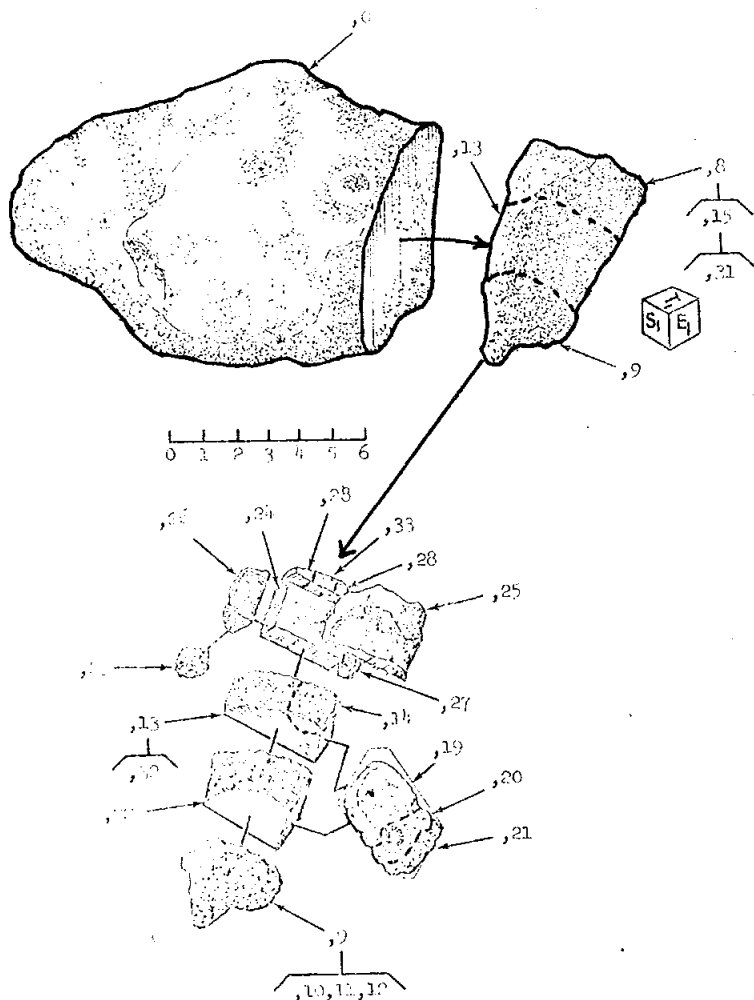
Figure 7. General subdivision of 15545.
